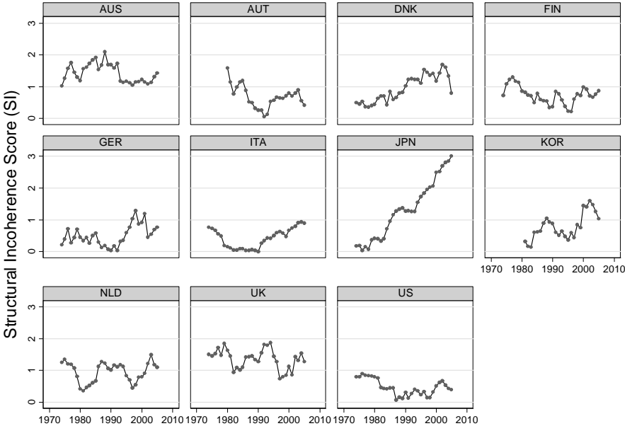
Figure 4: Evolution of structural incoherence score by country
